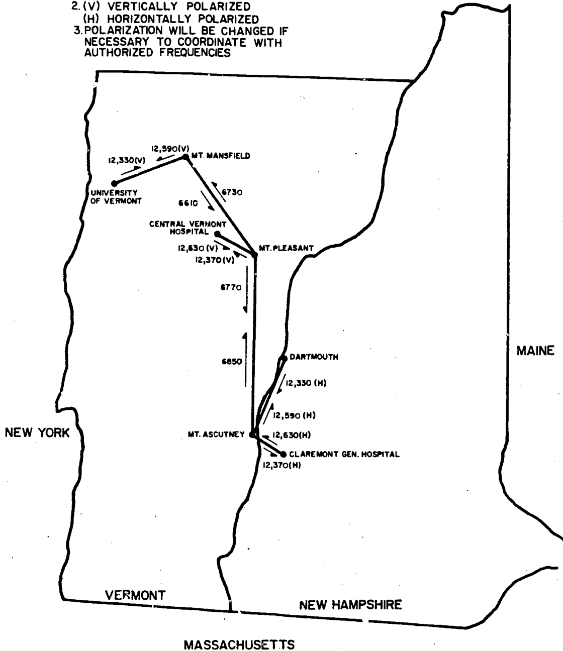
(b) FREQUENCY PLAN-VERMONT NEW HAMPSHIRE MEDICAL INTERACTIVE TELEVISION NETWORK
