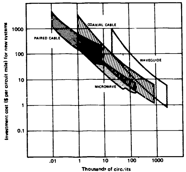
Costs of alternate methods of information transmission. Cost trends for terrestrial transmission of information are down while carrying capacity is up. Paired cable is the original telephone technology still in use; the others are later developments. The increases in the handling capacity of the four transmission systems represent developments over time as well as technical improvements. The investment costs are expressed as a range. This chart is adapted from staff papers prepared for the President's Task Force on Communications Policy, 1960.
